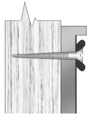
Wood Mount (Type D)
